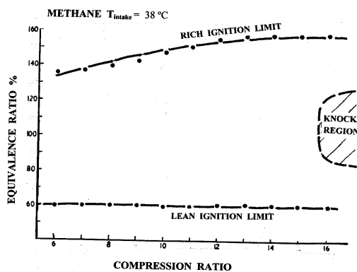
Figure (1) Variation of the Equivalence Ratio for the Ignition and Knock Limits with Compression Ratio for Methane at 38°C.
