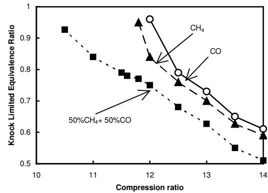
Figure (8) Variation of the Knock Limited Equivalence Ratio For CO, CH4 and (50% CO + 50% CH4) with Compression Ratio
