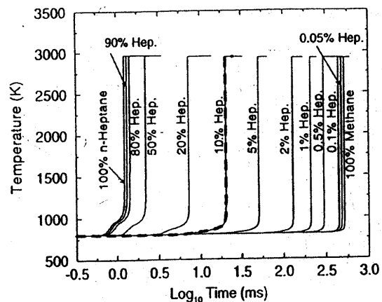
Figure (9) Variation of the Calculated Temperature Variation With Time For a Range of Additions of n-Heptane to Methane, (Khalil and Karim, 2002)
