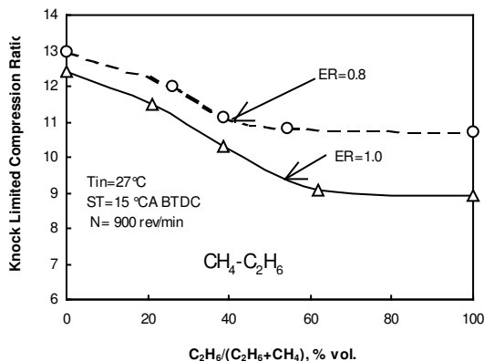
Figure (5) Variation of the Knock Limited Compression Ratio For Binary Mixtures of Methane and Ethane For Two Equivalence Ratios
