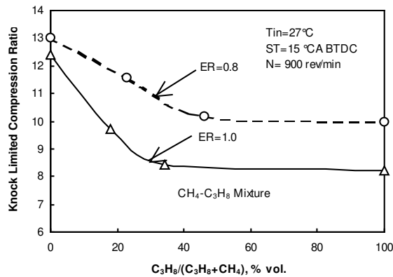
Figure (6) Variation of the Knock Limited Compression Ratio For Binary Mixtures of Propane and Methane For Two Equivalence Ratios
