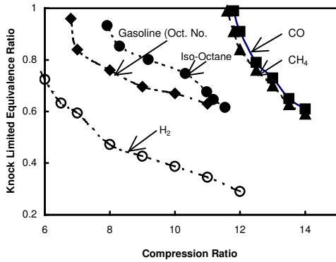
Figure (3) Variation of the Knock Limited Equivalence Ratio for CO, CH 4 , Isooctane, Gasoline and H 2 with Compression ratio
