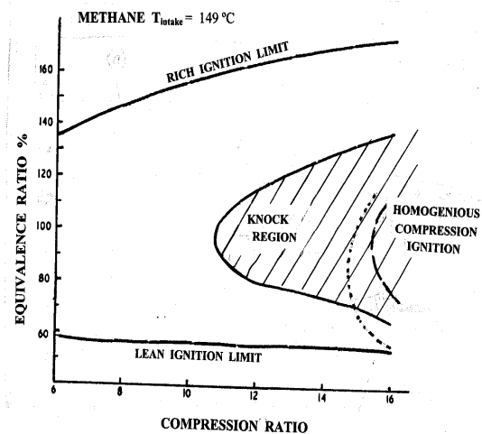
Figure (2) Variation of the Equivalence Ratio for the Ignition, Knock and Autoignition Limits with Compression Ratio for Methane at 149°C.
