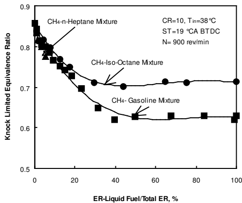
Figure (4) Variation of the Knock Limited Equivalence Ratio For Binary Mixtures of Methane with n-Heptane, iso-Octane and Gasoline
