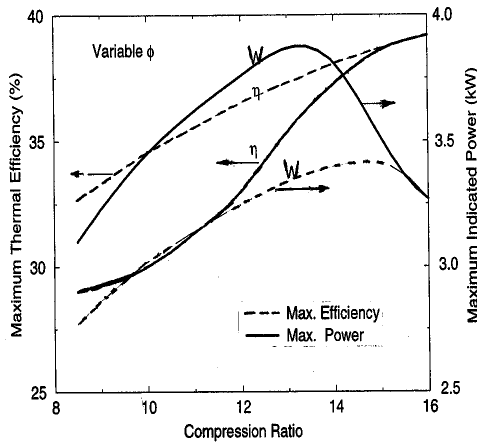
Figure (10) Variation of the Optimized Maximum Power Output and Maximum Efficiency Through Changing Equivalence Ratio With Compression Ratio- Methane Operation. (Attar and Karim, 2003)
