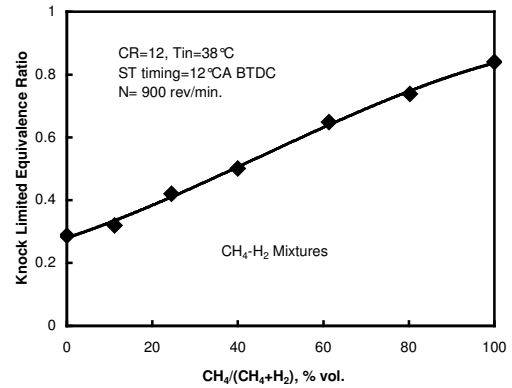
Figure (7) Variation of the Knock Limited Equivalence Ratio For Binary Mixture of Methane and Hydrogen at CR=12:1
